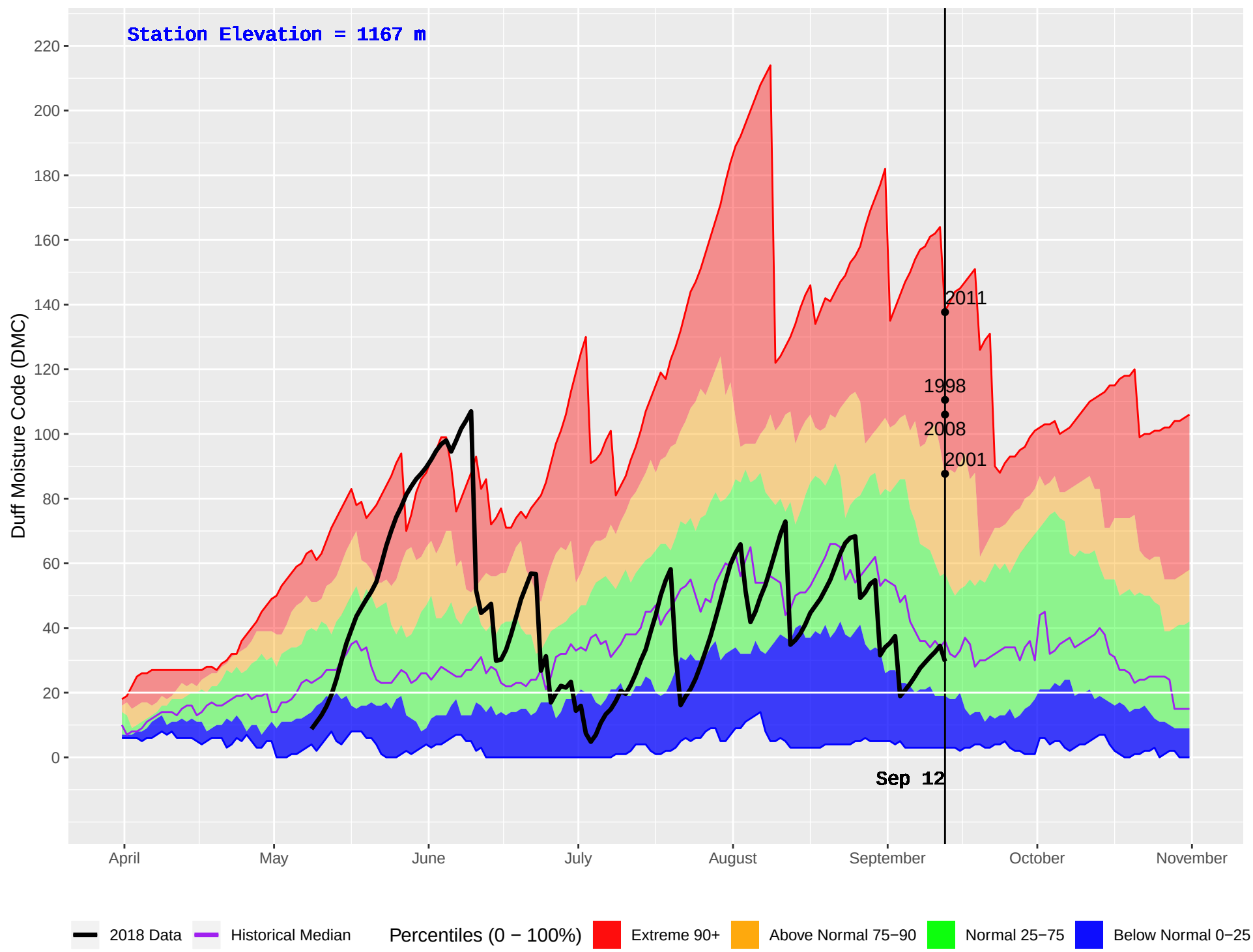
LEIGHTON LAKE (307) : Historical (1982–2016) and Current (2018) Daily Duff Moisture Code (DMC)
