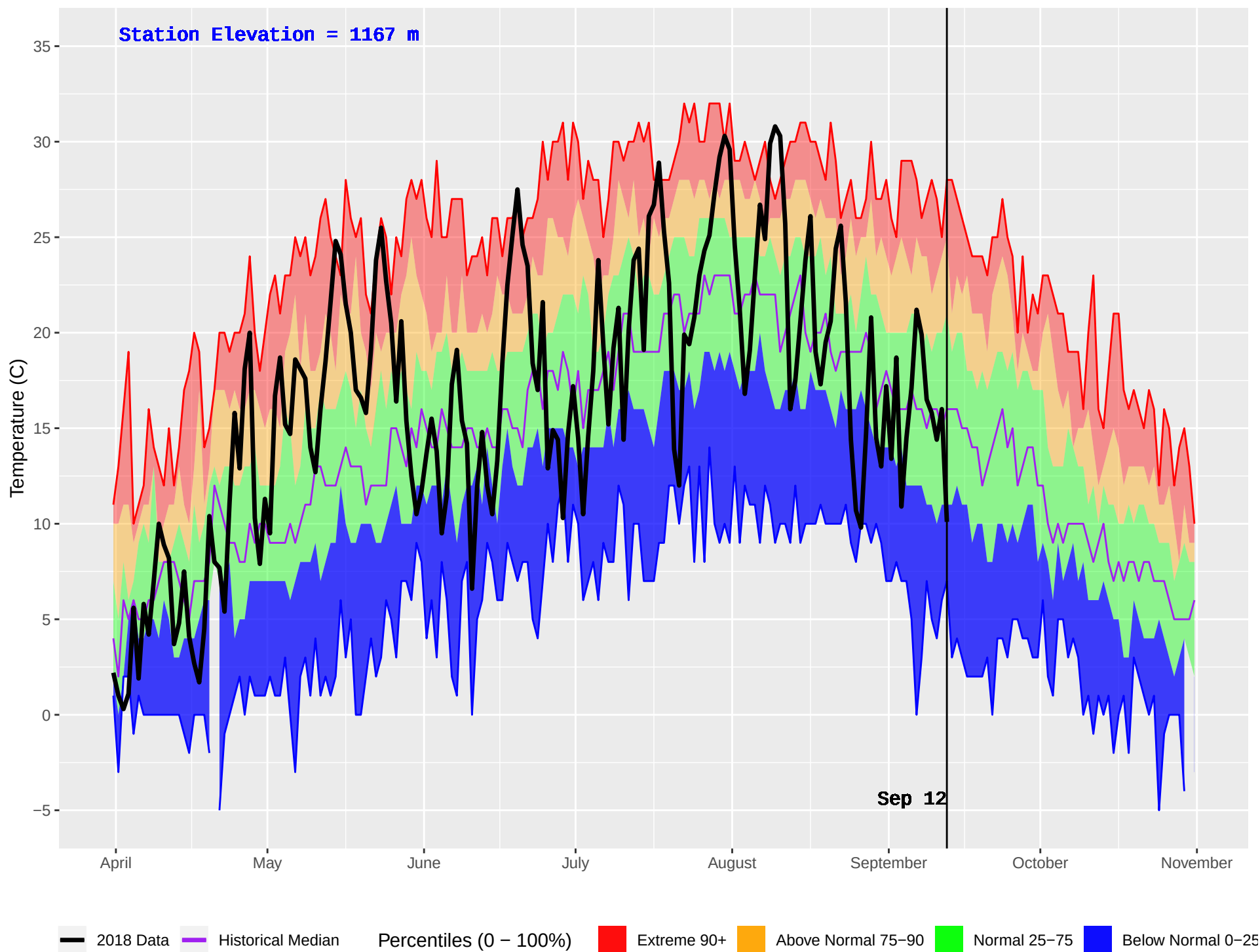
LEIGHTON LAKE (307) : Historical (1982–2016) and Current (2018) Daily Temperature
